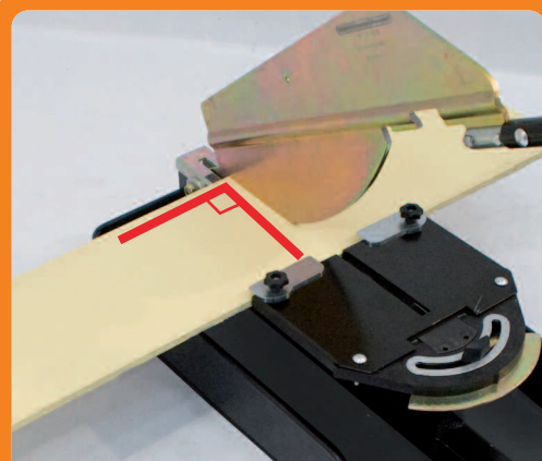
Angle cut 90°
